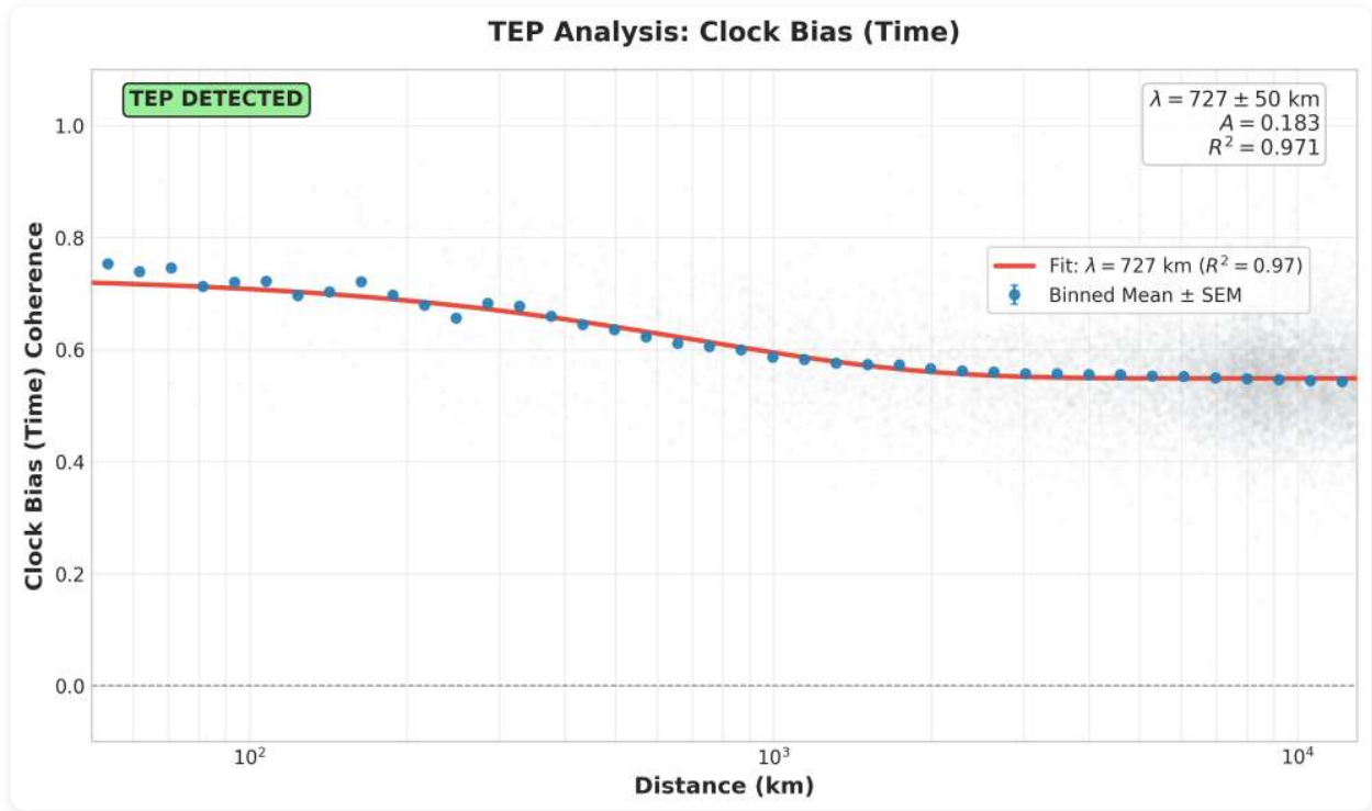
Figure 3.1: Phase coherence of clock bias between station pairs as a function of inter-station distance. Baseline GPS (L1) fit yields \lambda_T = 727 \pm 50 \text{ km} with R^2 = 0.971 . Error bars represent standard error of the mean within each distance bin.
