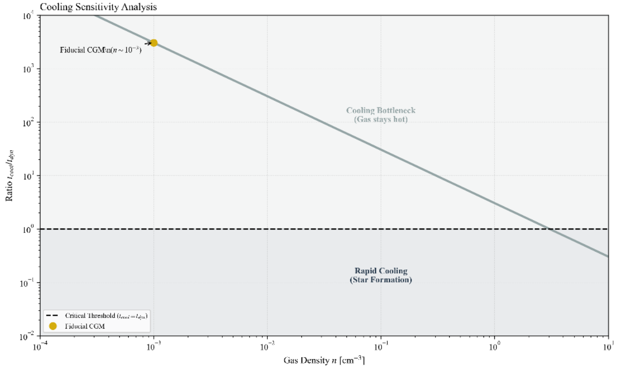
Figure 2: Cooling Sensitivity Analysis. The ratio of cooling time to dynamical time ( t_{\text{cool}}/t_{\text{dyn}} ) as a function of gas density. For standard CGM densities ( n \sim 10^{-3} \text{ cm}^{-3} ), the ratio is \gg 1 , indicating a cooling bottleneck.
